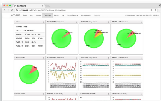
Dashboard page showing system data and statistic chart
