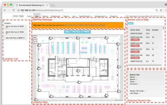
Real-time Map view showing all tags and readers deployed
